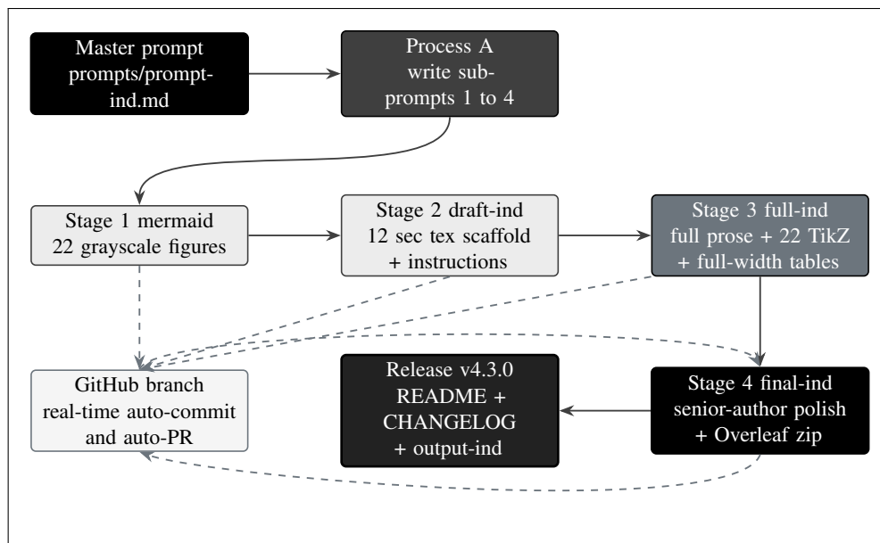
Figure 1. The single-prompt mermaid to draft to full to final build pipeline for the Phase 1 PDAC IND. One master prompt drives Process A (write the four sub-prompts) and then Process B (execute them as Stages 1 to 4). Dashed edges show that every generated file is committed and pushed to one continuously updated pull request in real time, and the feedback edge shows author review returning into the final stage, all without manual intervention.
